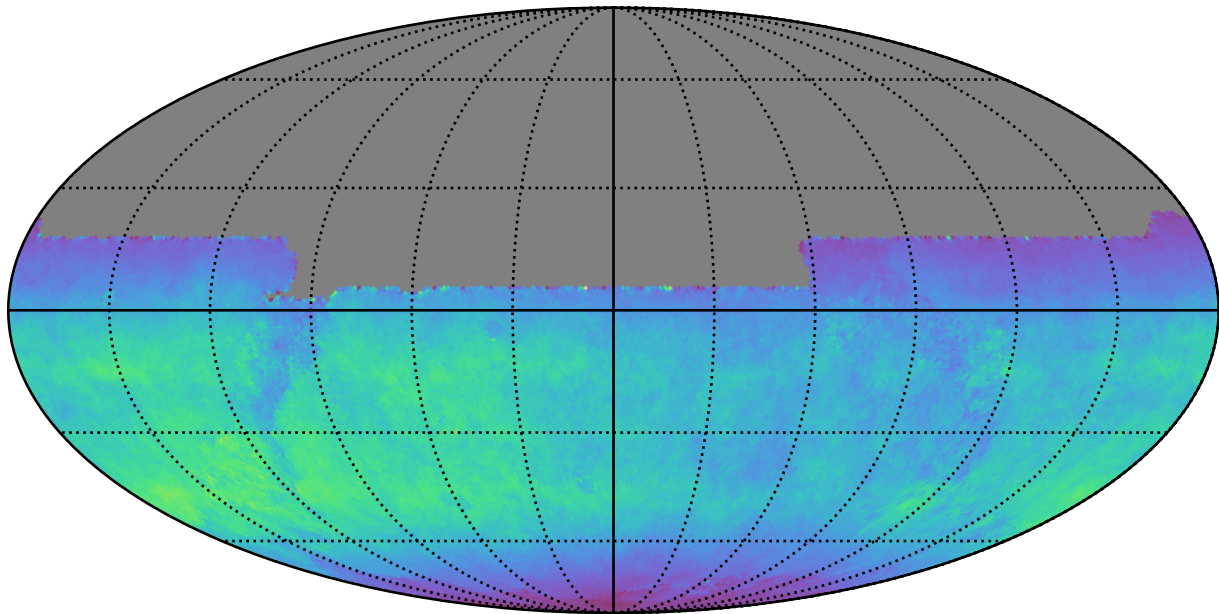
too_elab_r256_d2_gz_v3.4_10yrs All sky y band: Normalized Teff
