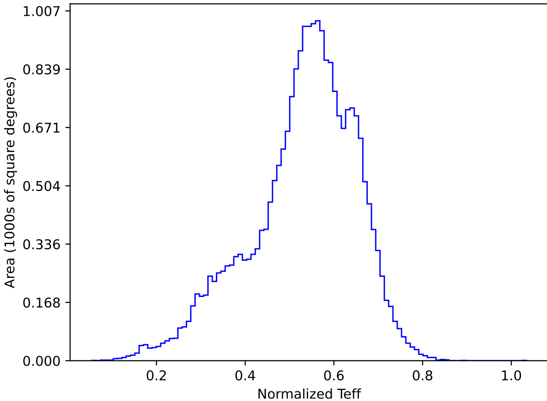
too_elab_r256_d2_gz_v3.4_10yrs All sky y band: Normalized Teff
