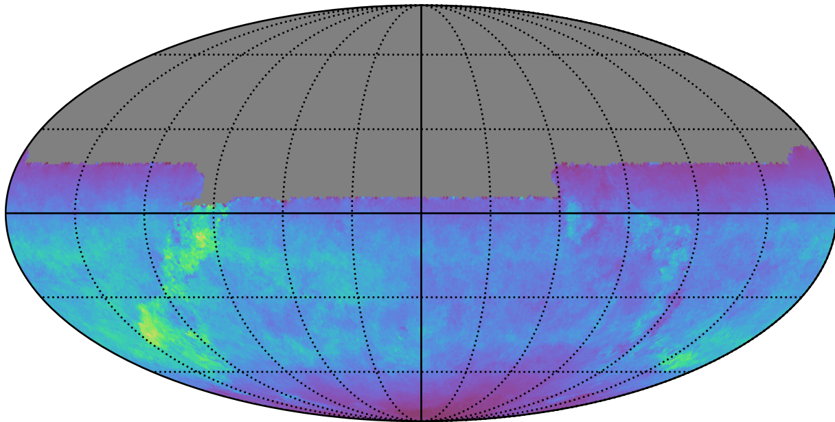
too_elab_r256_d2_gz_v3.4_10yrs All sky u band: Normalized Teff
