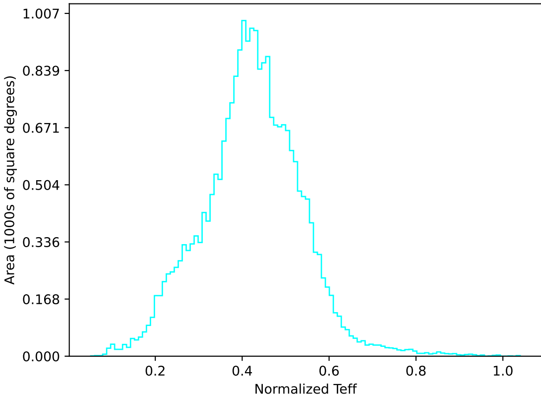
too_elab_r256_d2_gz_v3.4_10yrs All sky u band: Normalized Teff
