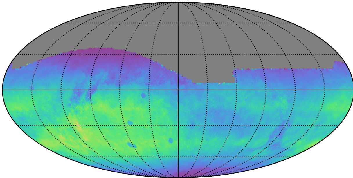
too_elab_r256_d2_gz_v3.4_10yrs All sky r band: Normalized Teff
