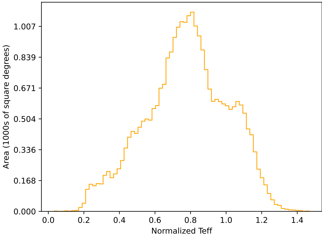
too_elab_r256_d2_gz_v3.4_10yrs All sky r band: Normalized Teff
