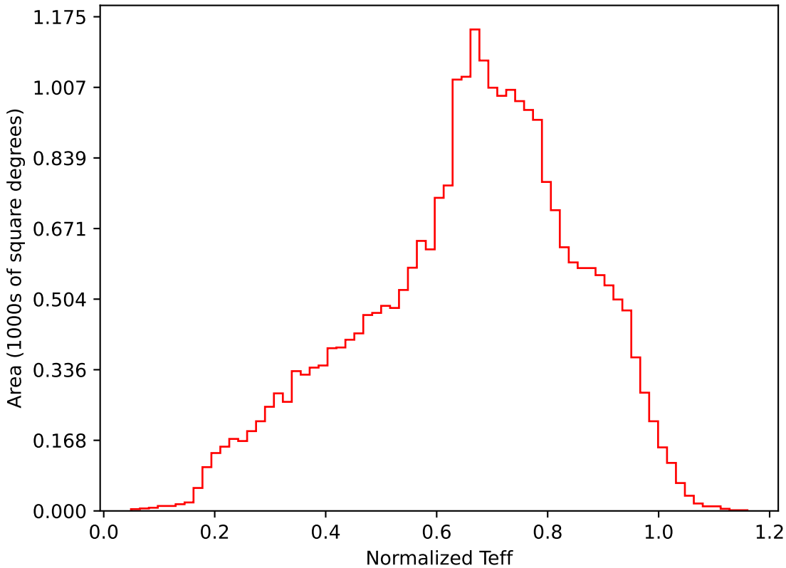
too_elab_r256_d2_gz_v3.4_10yrs All sky i band: Normalized Teff
