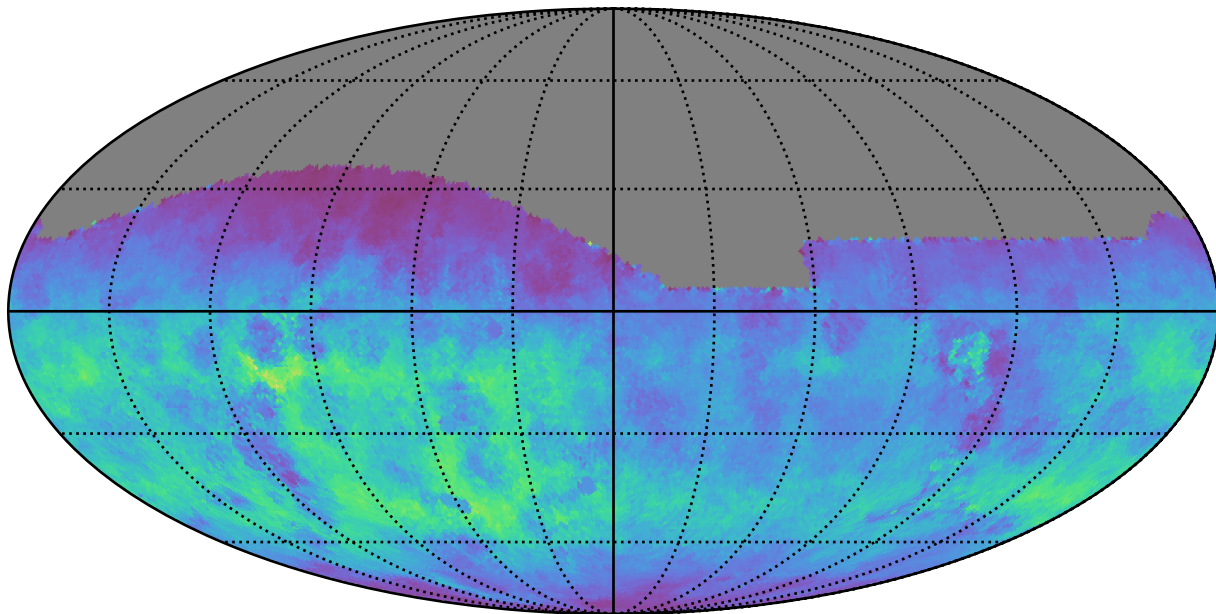
too_elab_r256_d2_gz_v3.4_10yrs All sky g band: Normalized Teff
