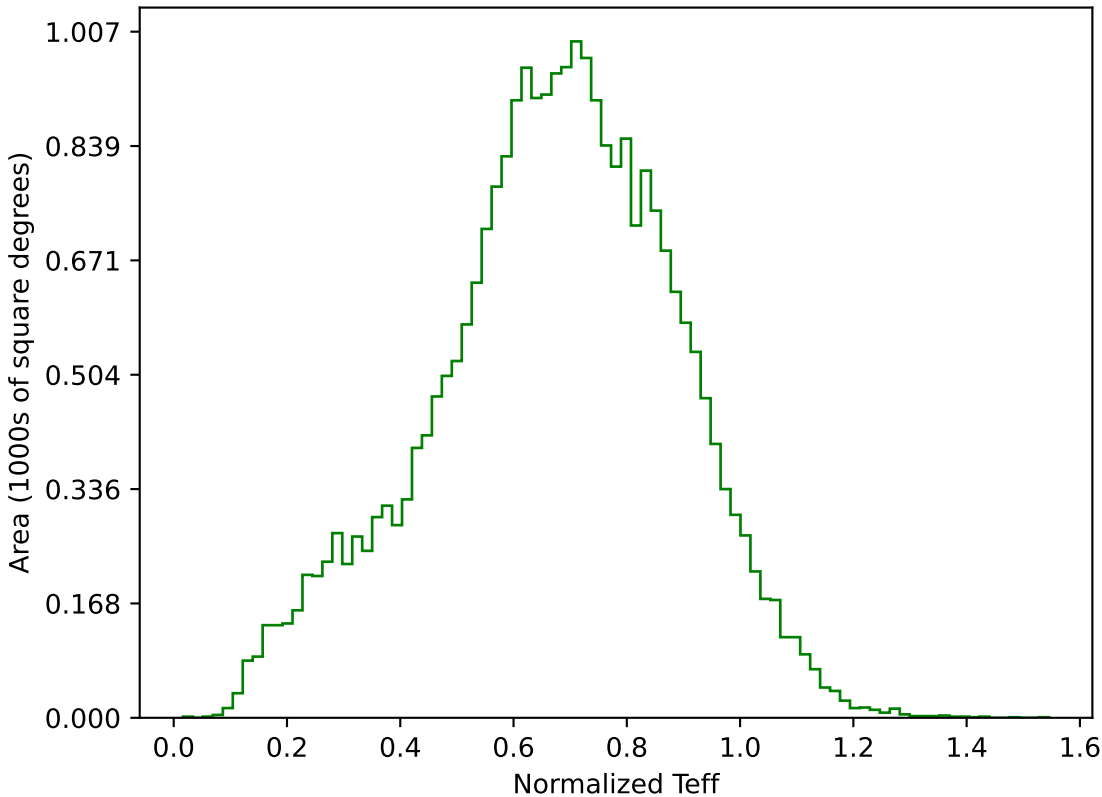
too_elab_r256_d2_gz_v3.4_10yrs All sky g band: Normalized Teff
