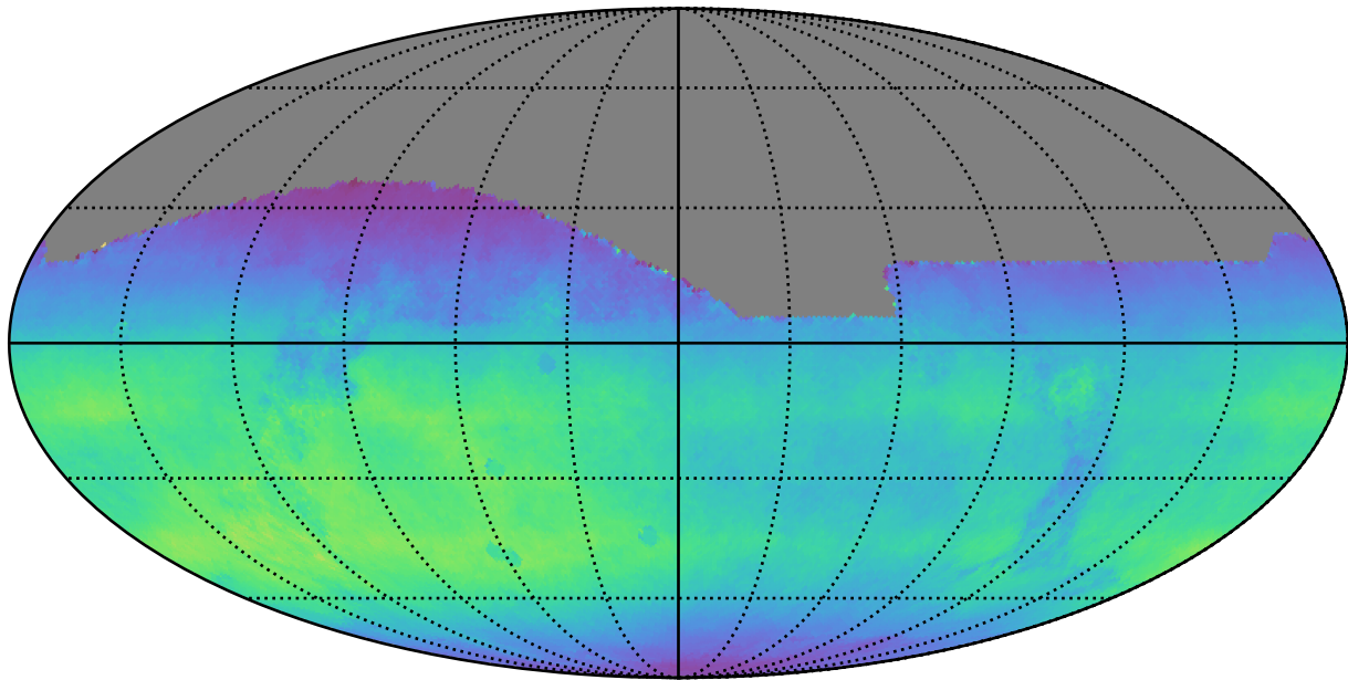
too_elab_r256_d2_gz_v3.4_10yrs All sky all bands: Normalized Teff
