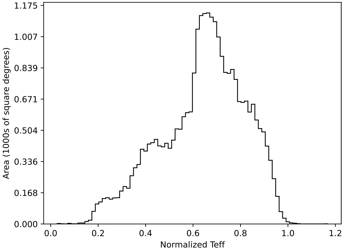
too_elab_r256_d2_gz_v3.4_10yrs All sky all bands: Normalized Teff
