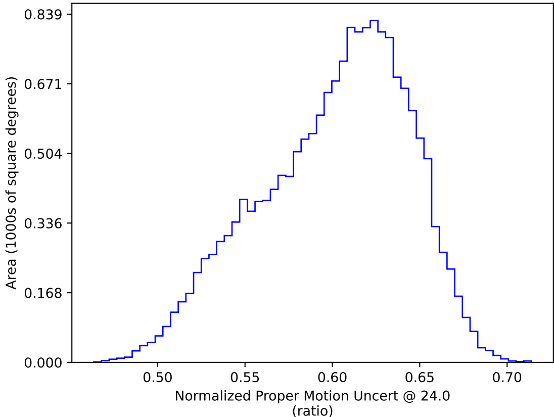
too_elab_r256_d2_gz_v3.4_10yrs WFD: Normalized Proper Motion Uncert @ 24.0
