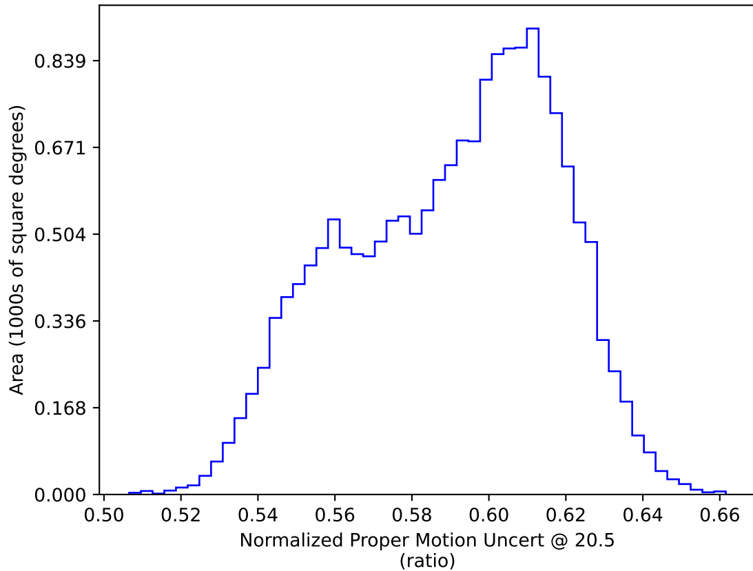
too_elab_r256_d2_gz_v3.4_10yrs WFD: Normalized Proper Motion Uncert @ 20.5
