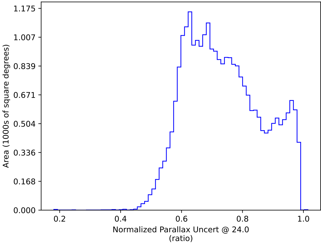
too_elab_r256_d2_gz_v3.4_10yrs All sky: Normalized Parallax Uncert @ 24.0
