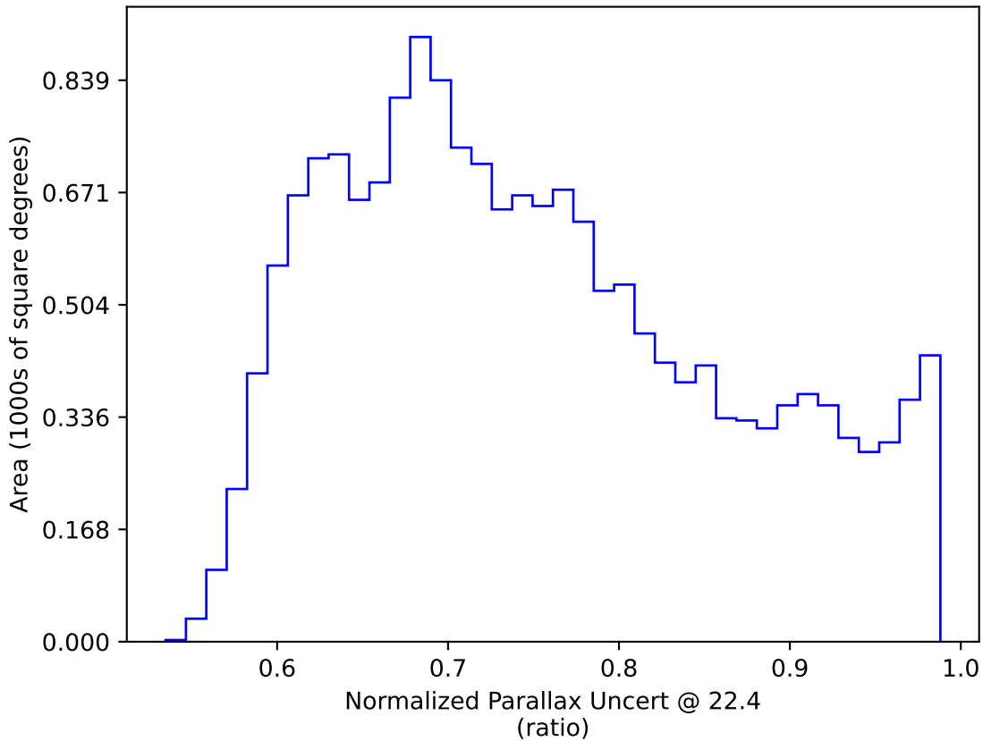
too_elab_r256_d2_gz_v3.4_10yrs WFD: Normalized Parallax Uncert @ 22.4
