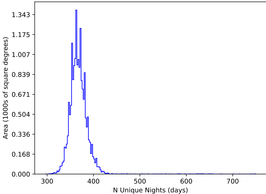
too_elab_r256_d2_gz_v3.4_10yrs WFD all bands: N Unique Nights
