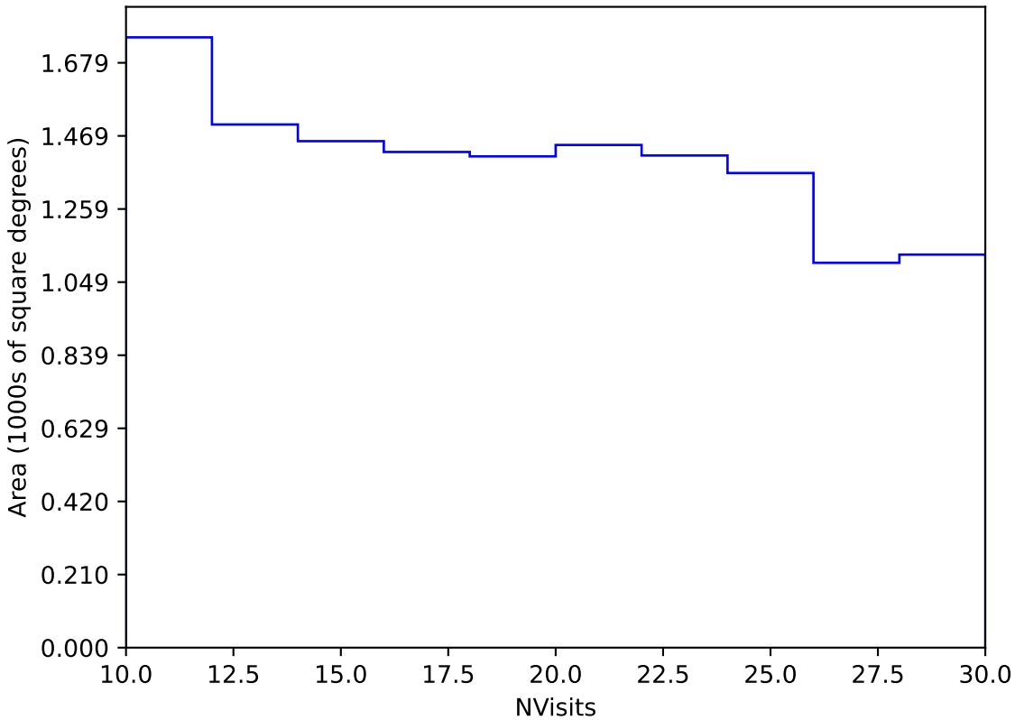
too_elab_r256_d2_gz_v3.4_10yrs Yr 3-4 y band: NVisits
