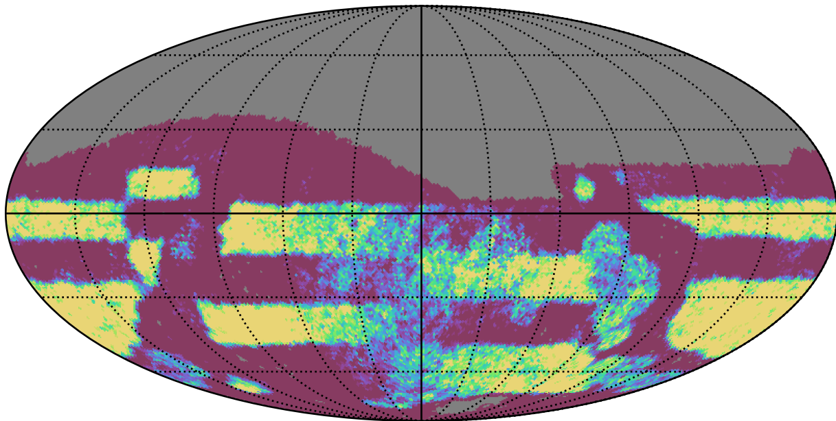
too_elab_r256_d2_gz_v3.4_10yrs Yr 3-4 r band: NVisits
