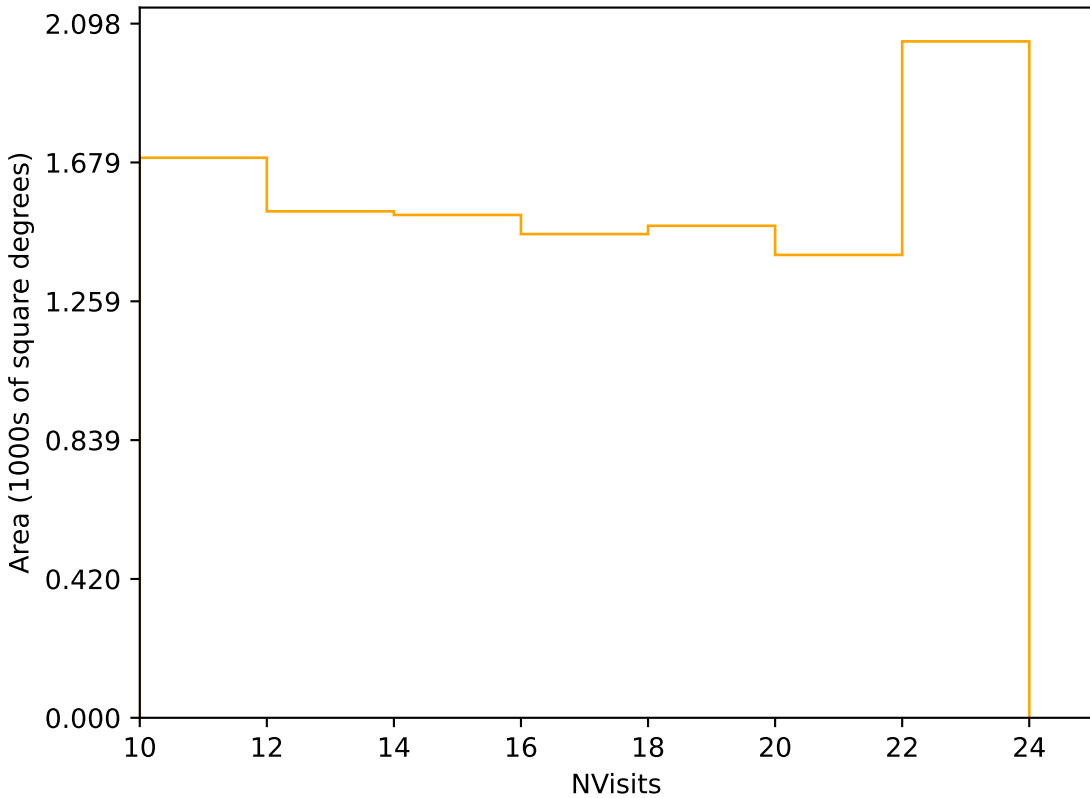
too_elab_r256_d2_gz_v3.4_10yrs Yr 3-4 r band: NVisits
