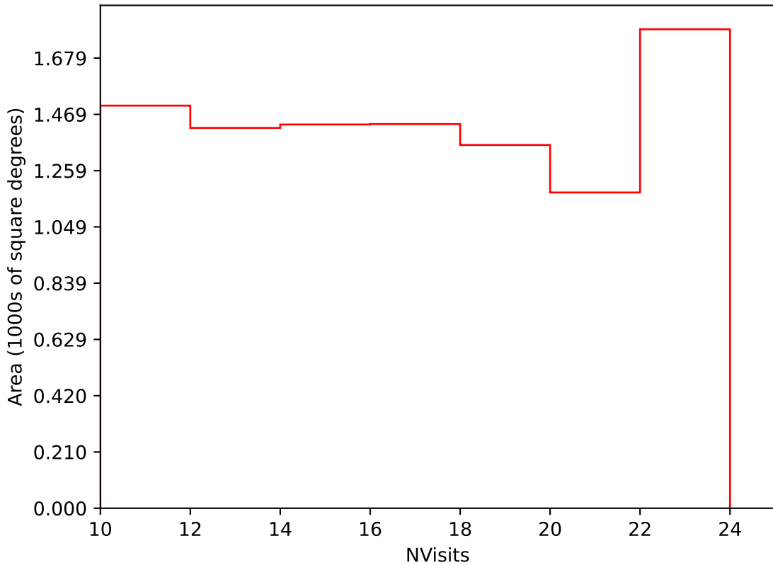
too_elab_r256_d2_gz_v3.4_10yrs Yr 3-4 i band: NVisits
