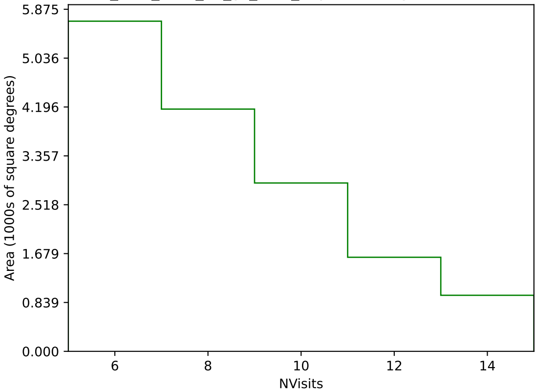
too_elab_r256_d2_gz_v3.4_10yrs Yr 3-4 g band: NVisits
