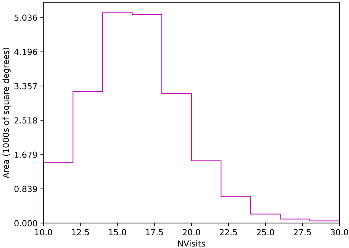
too_elab_r256_d2_gz_v3.4_10yrs Yr 1 z band: NVisits
