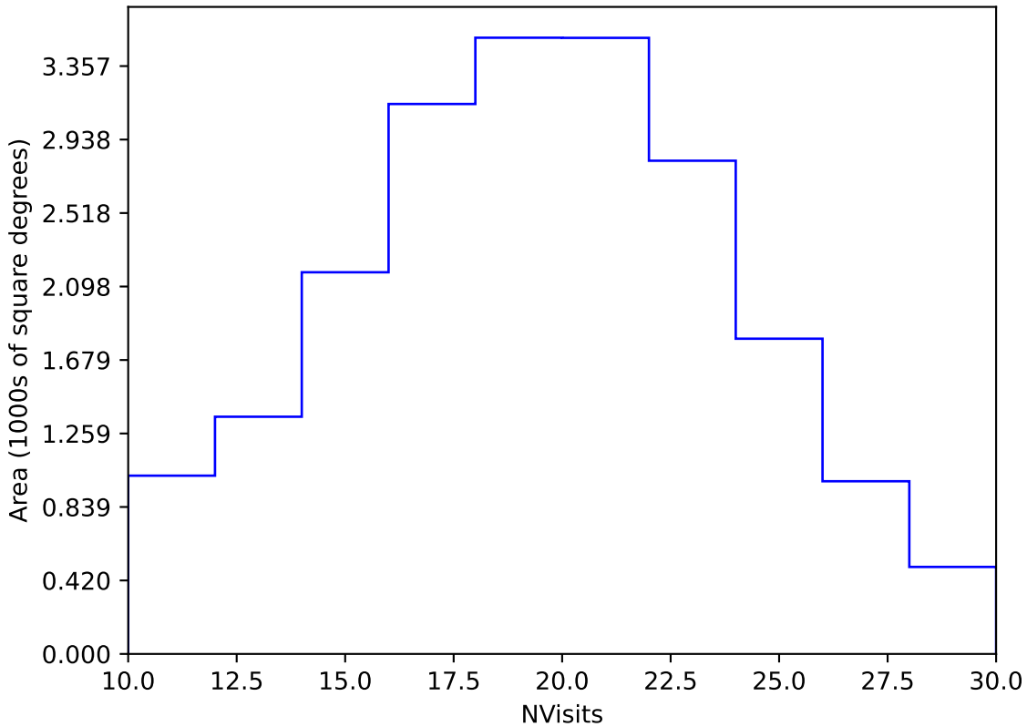
too_elab_r256_d2_gz_v3.4_10yrs Yr 1 y band: NVisits
