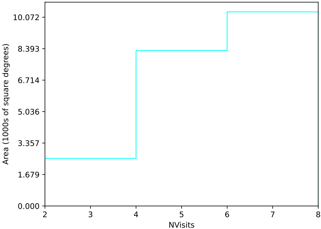
too_elab_r256_d2_gz_v3.4_10yrs Yr 1 u band: NVisits
