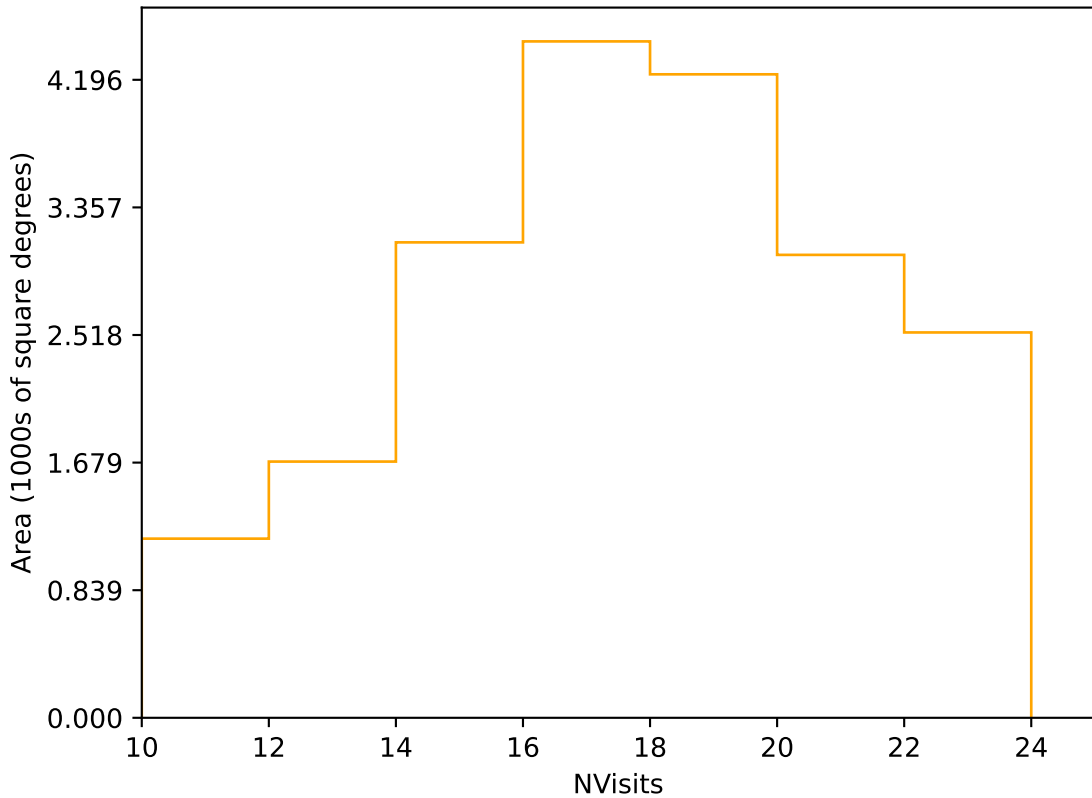
too_elab_r256_d2_gz_v3.4_10yrs Yr 1 r band: NVisits
