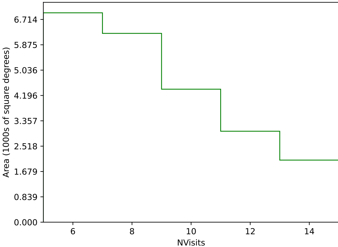
too_elab_r256_d2_gz_v3.4_10yrs Yr 1 g band: NVisits
