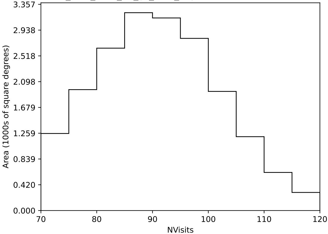
too_elab_r256_d2_gz_v3.4_10yrs Yr 1 all bands: NVisits
