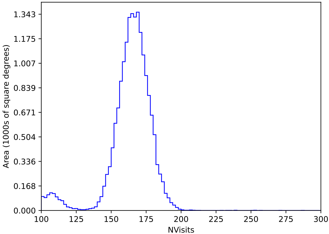
too_elab_r256_d2_gz_v3.4_10yrs WFD y band: NVisits
