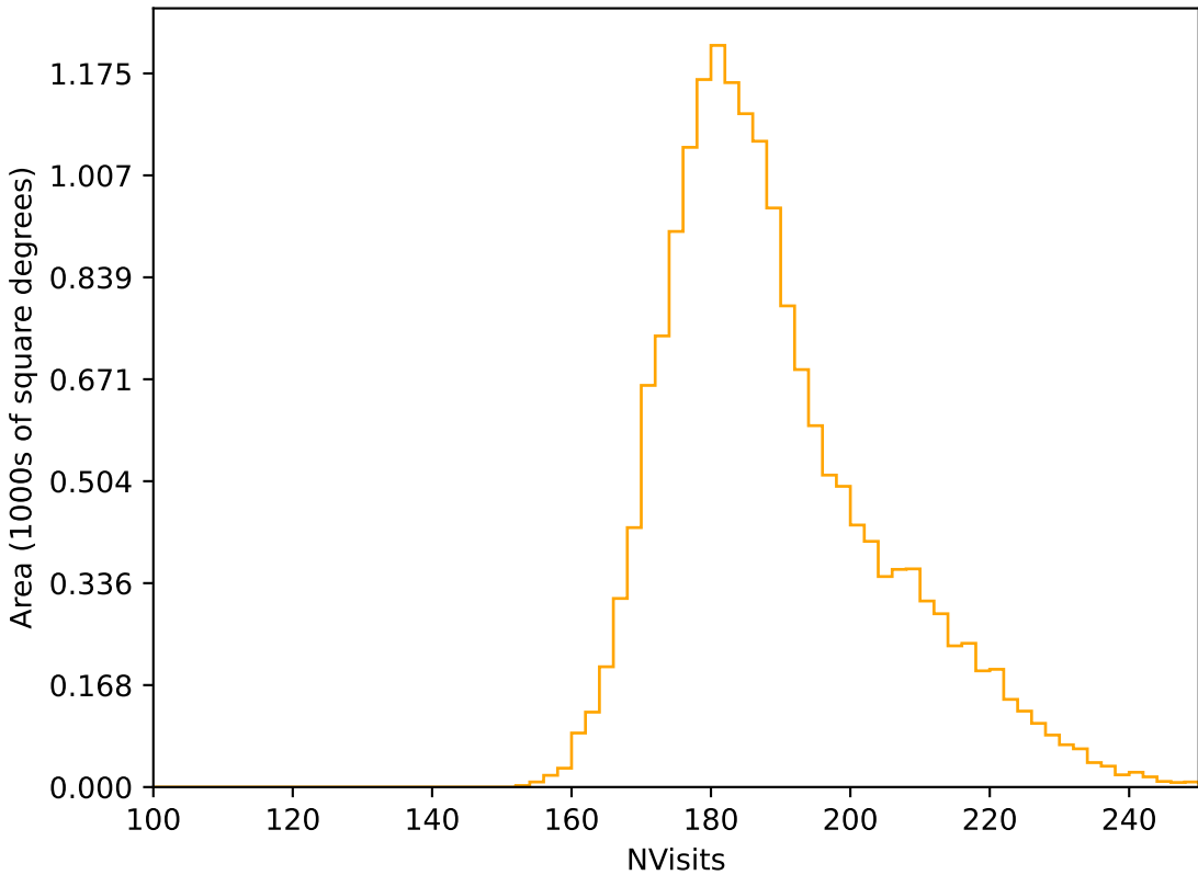
too_elab_r256_d2_gz_v3.4_10yrs WFD r band: NVisits
