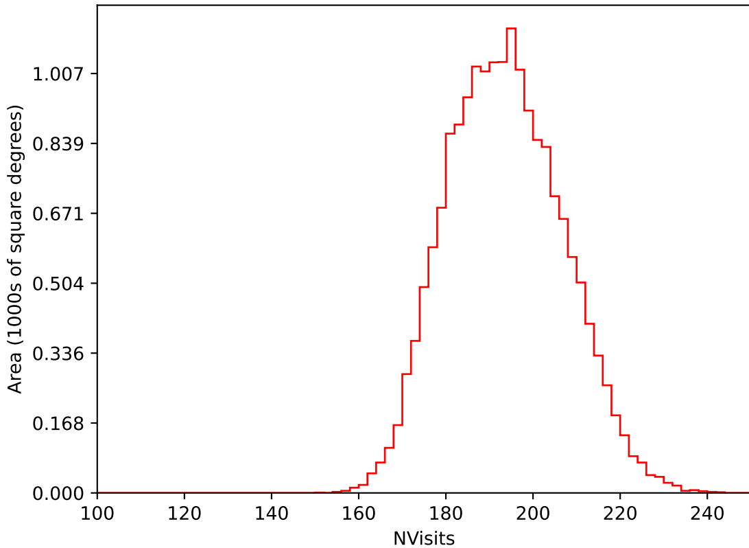
too_elab_r256_d2_gz_v3.4_10yrs WFD i band: NVisits
