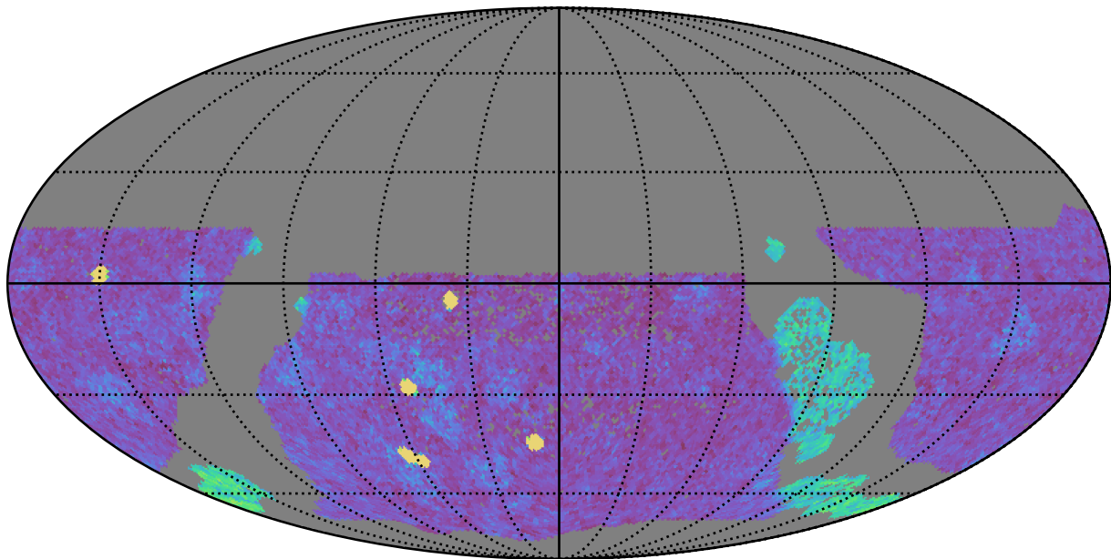
too_elab_r256_d2_gz_v3.4_10yrs WFD g band: NVisits
