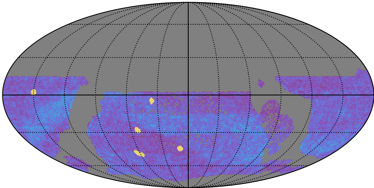
too_elab_r256_d2_gz_v3.4_10yrs WFD all bands: NVisits
