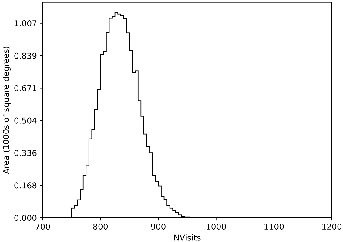
too_elab_r256_d2_gz_v3.4_10yrs WFD all bands: NVisits
