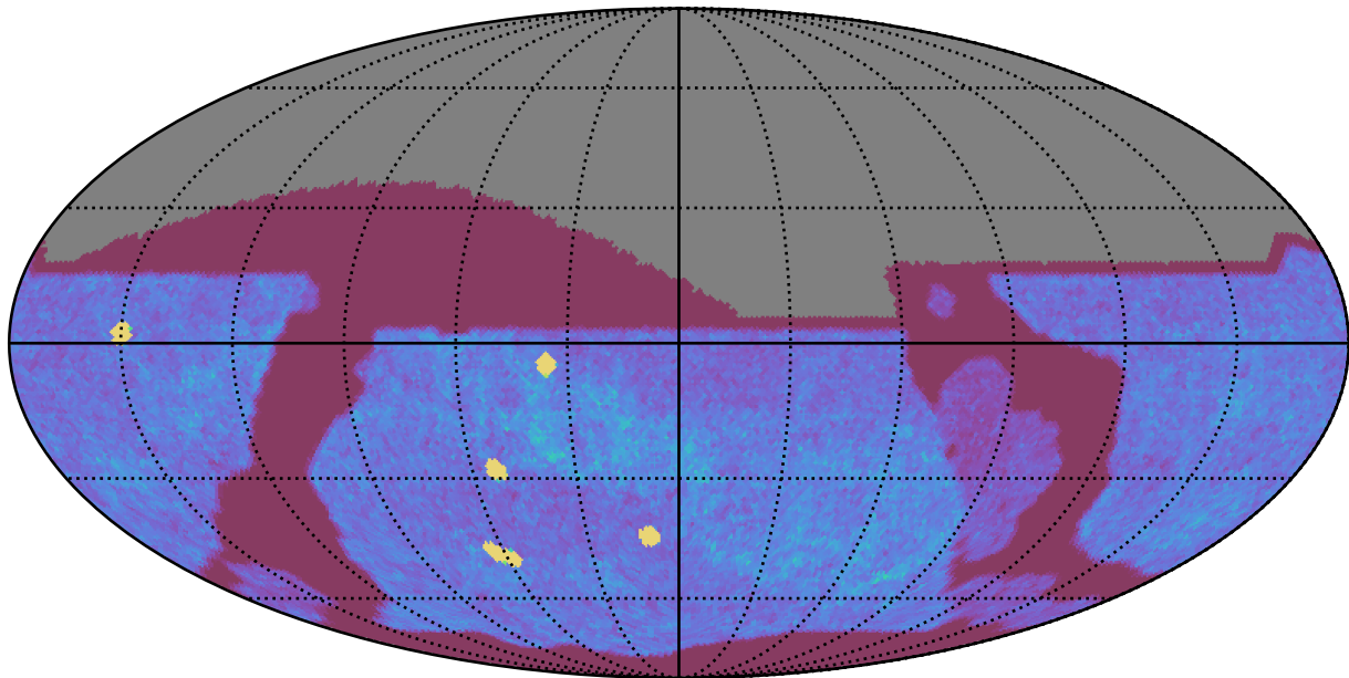
too_elab_r256_d2_gz_v3.4_10yrs All sky z band: NVisits
