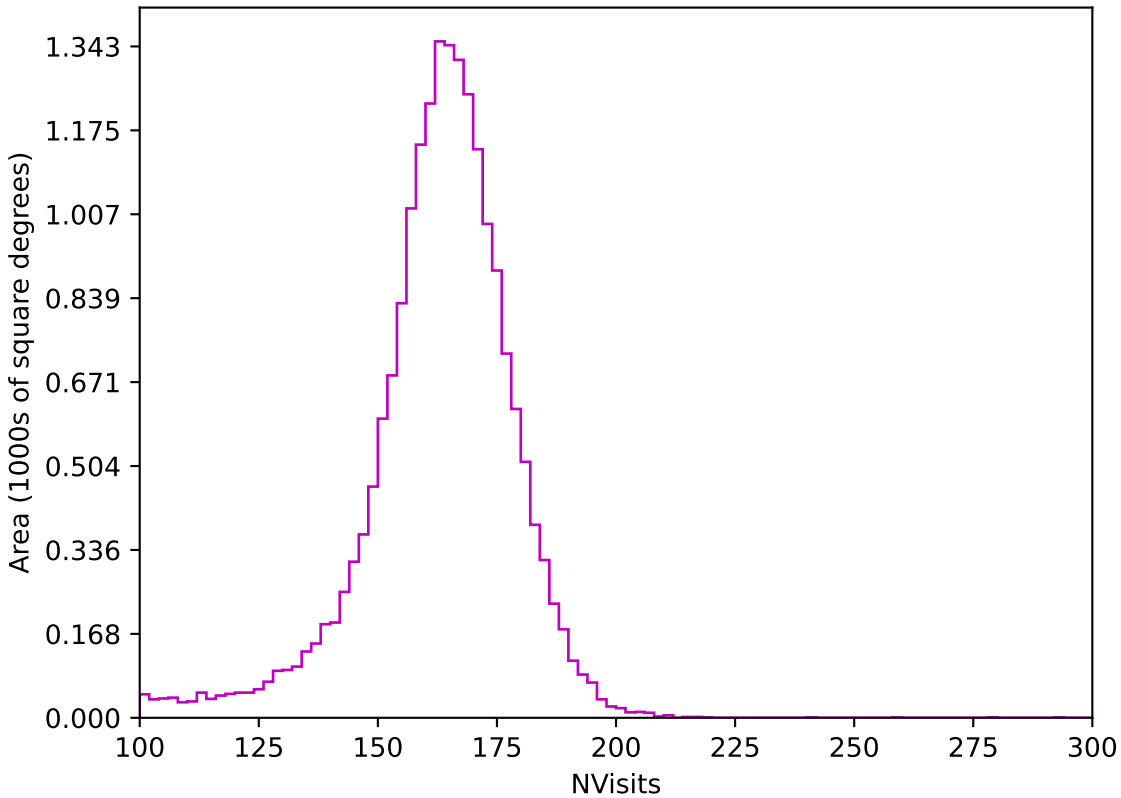
too_elab_r256_d2_gz_v3.4_10yrs All sky z band: NVisits
