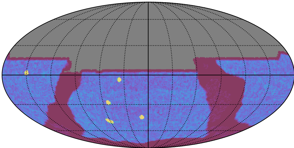
too_elab_r256_d2_gz_v3.4_10yrs All sky y band: NVisits
