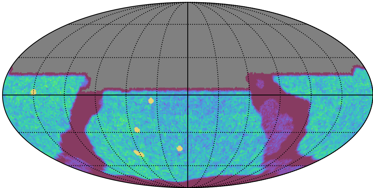
too_elab_r256_d2_gz_v3.4_10yrs All sky u band: NVisits
