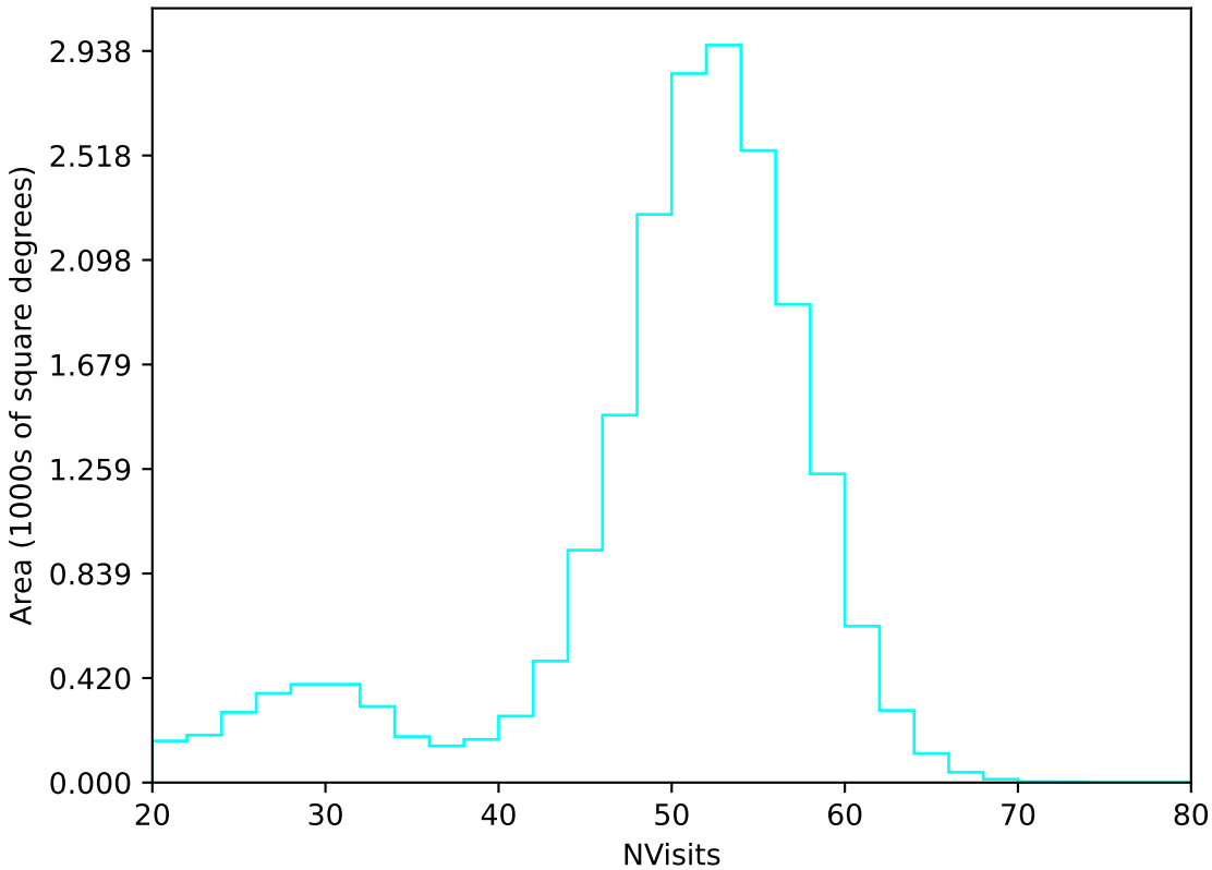
too_elab_r256_d2_gz_v3.4_10yrs All sky u band: NVisits
