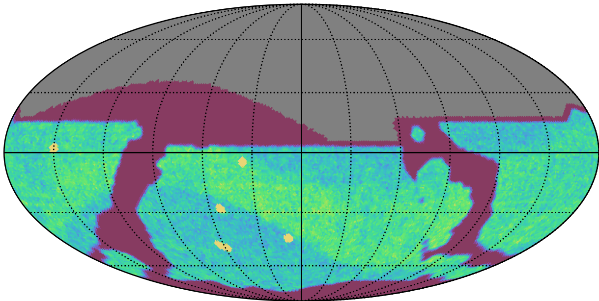
too_elab_r256_d2_gz_v3.4_10yrs All sky i band: NVisits
