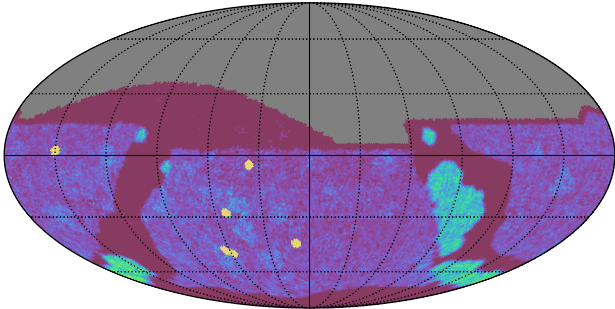
too_elab_r256_d2_gz_v3.4_10yrs All sky g band: NVisits
