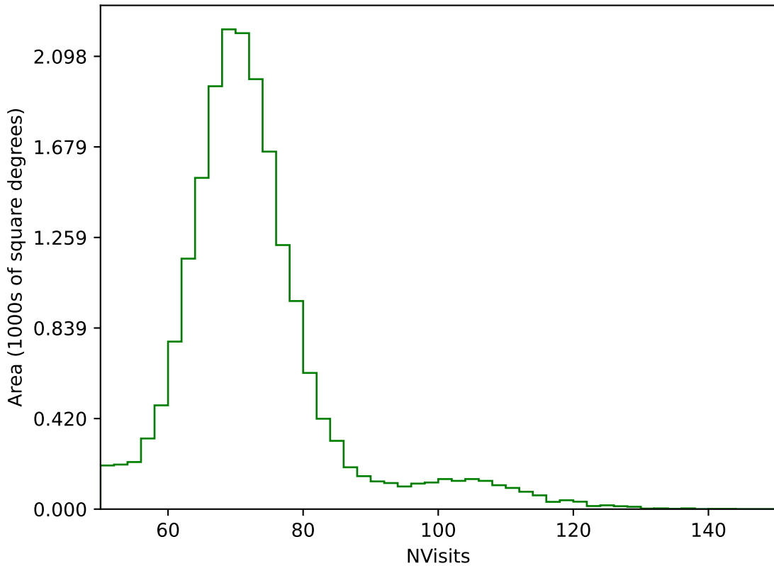
too_elab_r256_d2_gz_v3.4_10yrs All sky g band: NVisits
