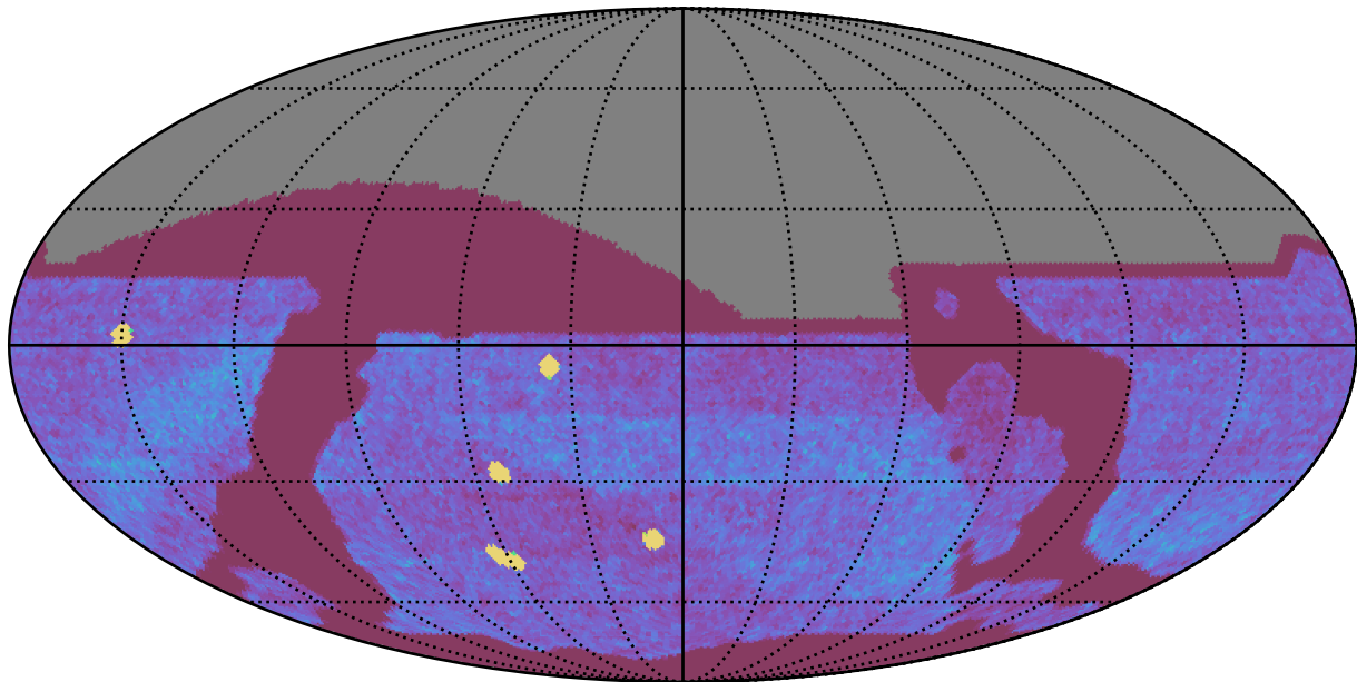
too_elab_r256_d2_gz_v3.4_10yrs All sky all bands: NVisits
