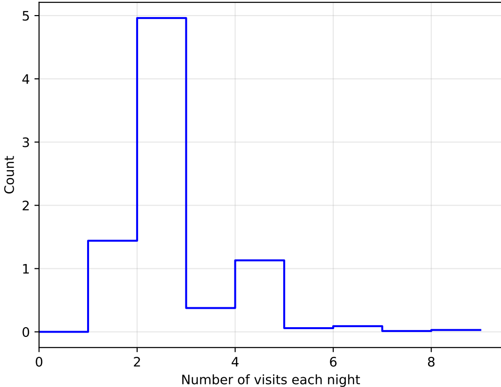
too_elab_r256_d2_gz_v3.4_10yrs WFD: NVisitsPerNight
