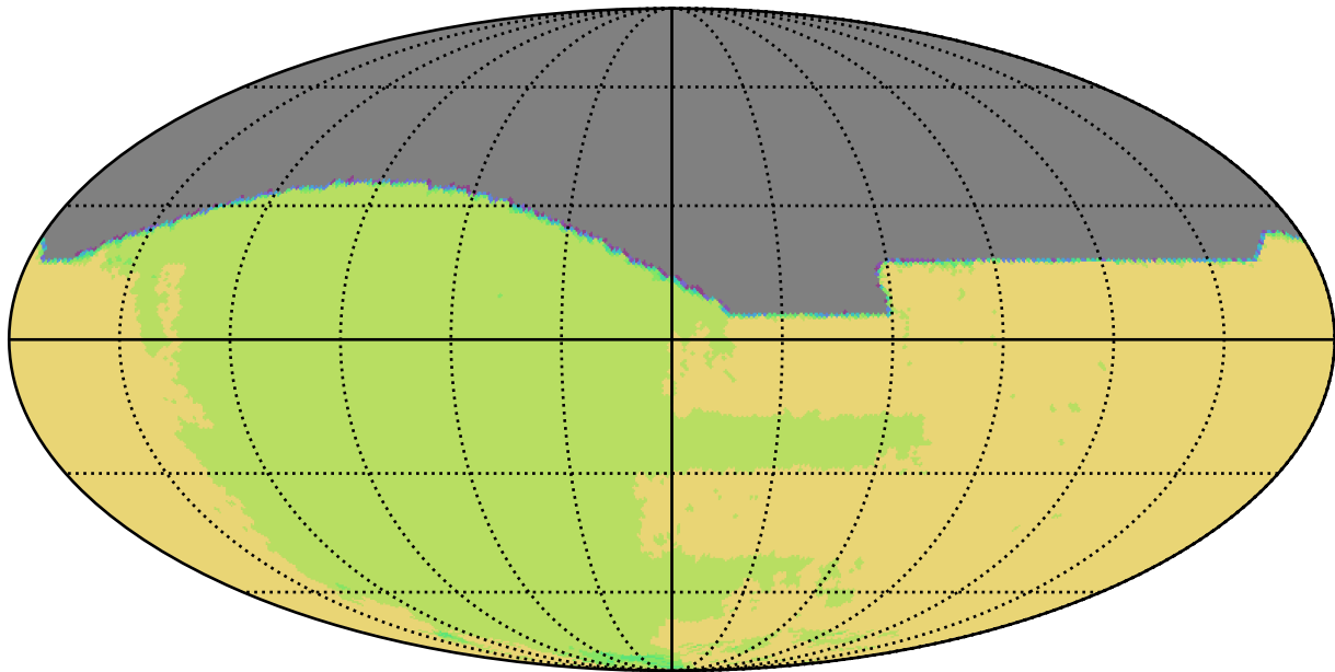
too_elab_r256_d2_gz_v3.4_10yrs All sky all bands: NSeasons
