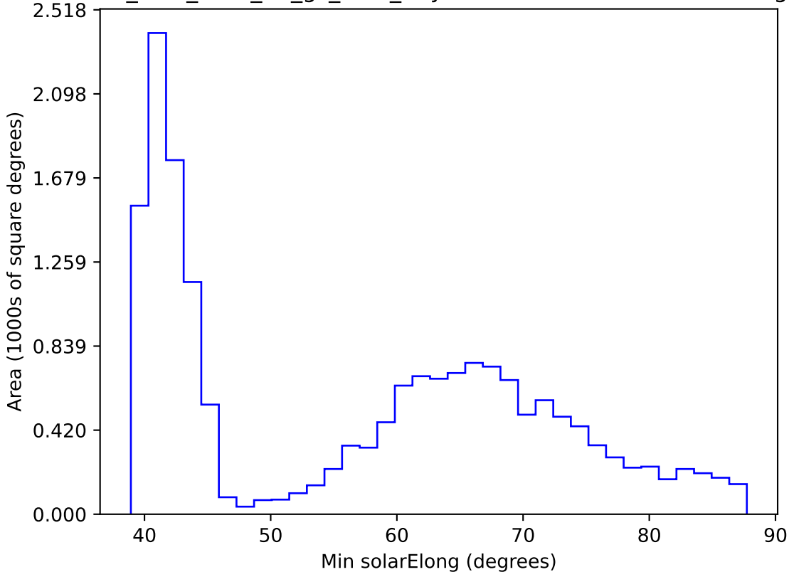
too_elab_r256_d2_gz_v3.4_10yrs WFD r band: Min solarElong
