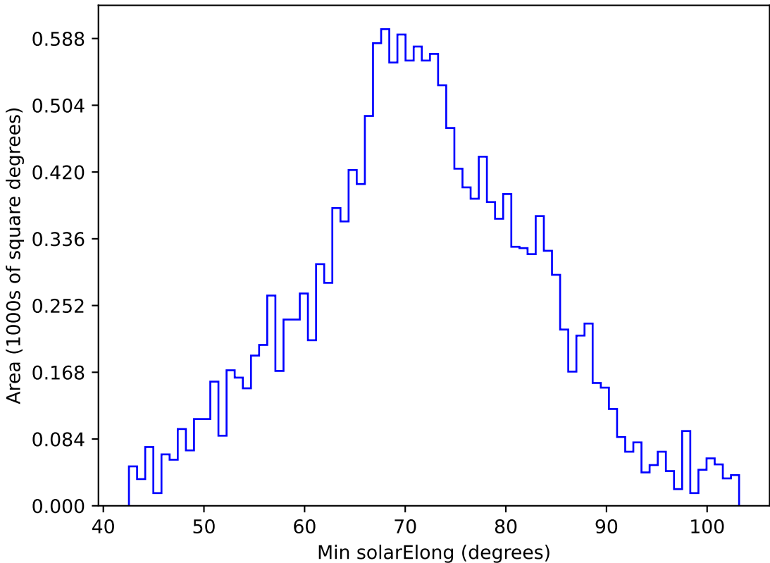
too_elab_r256_d2_gz_v3.4_10yrs WFD g band: Min solarElong
