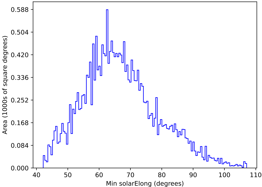
too_elab_r256_d2_gz_v3.4_10yrs All sky y band: Min solarElong
