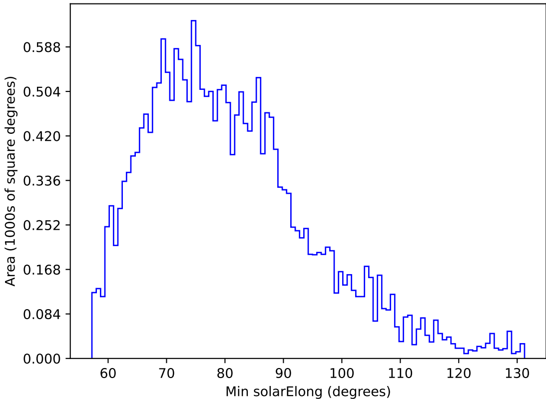
too_elab_r256_d2_gz_v3.4_10yrs All sky u band: Min solarElong
