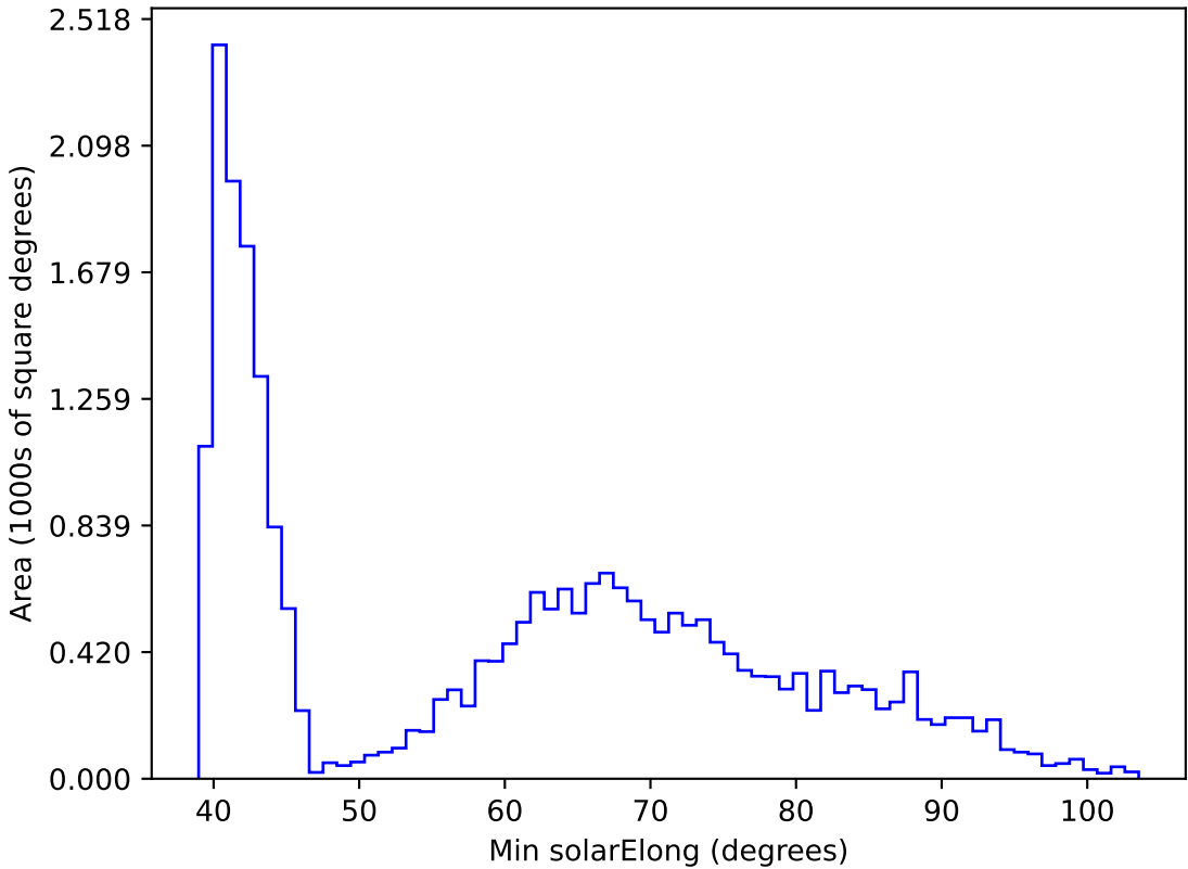
too_elab_r256_d2_gz_v3.4_10yrs All sky r band: Min solarElong
