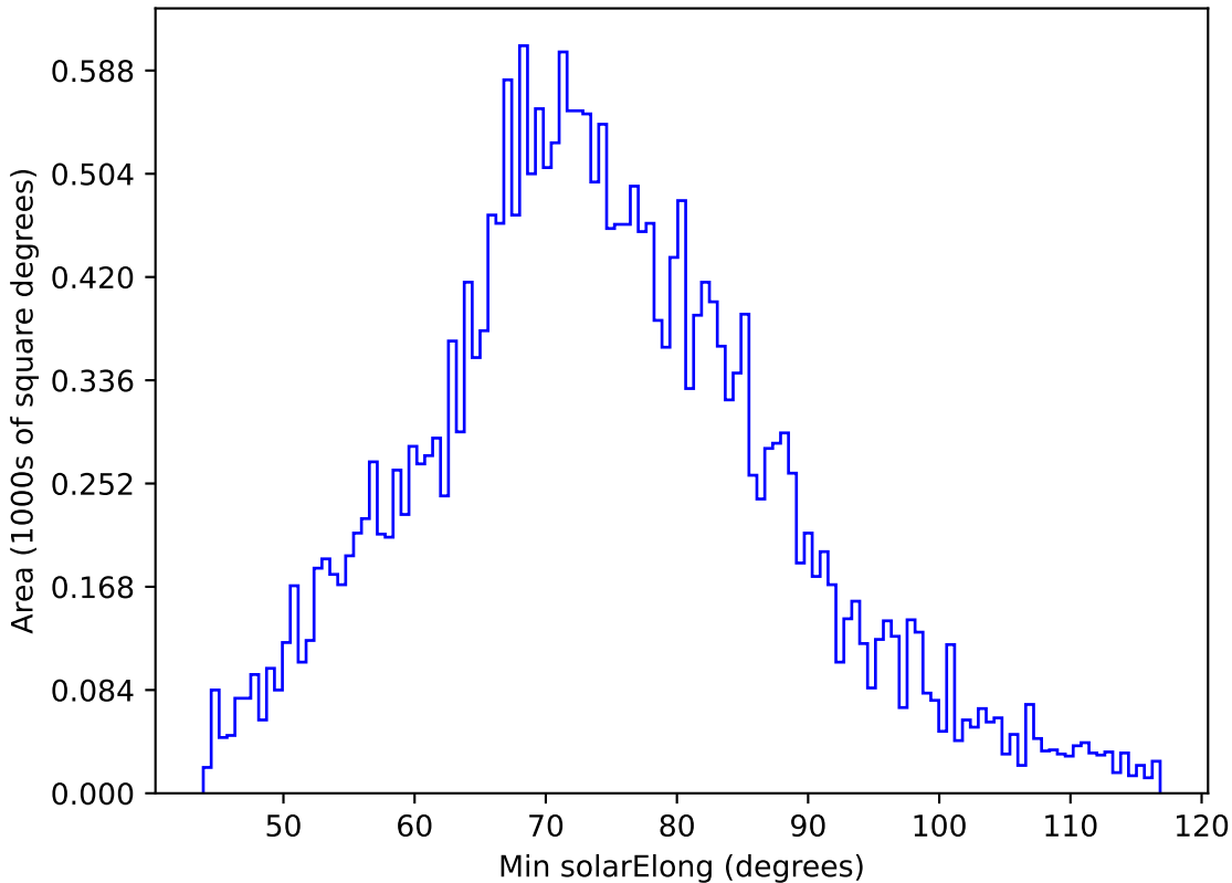
too_elab_r256_d2_gz_v3.4_10yrs All sky g band: Min solarElong
